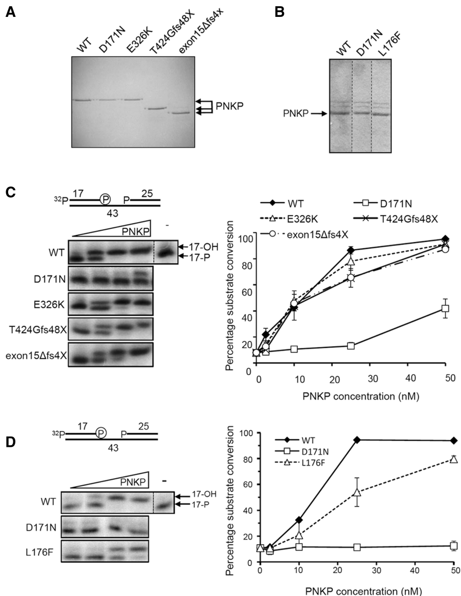
Figure 2. DNA 3'-phosphatase activity of recombinant PNKP harbouring mutations associated with MCSZ. (A and B) Aliquots of the recombinant WT and mutant human PNKP (0.7–1 μg) employed in these experiments was fractionated by SDS-PAGE and visualized by staining with Coomassie brilliant blue. Note that the PNKP proteins depicted in panel A were purified by IMAC/cation exchange and employed in panel C, below, whereas those depicted in panel B were purified by IMAC alone and employed in panel D, below. (C and D) DNA 3'-phosphatase activities of WT and mutant PNKP. 25 nM of the indicated oligonucleotide duplex substrate (top) was incubated without (–) or with 2.5, 10, 25 or 50 nM of WT or the indicated mutant PNKP protein for 60 min at 30°C. Reaction products were fractionated by denaturing PAGE and detected by phosphorimaging. A representative gel is shown on the left, and quantification from four independent experiments (±SEM) on the right. For quantification, the signal intensities of the 17-P substrate and 17-OH product bands were quantified using Aida Image Analyser v.427 and the percentage of 17-OH product calculated. The oligonucleotide duplex contains a 1-bp gap with 3'-phosphate and 5'-phosphate termini. The position of the 3'-phosphate (circled) and 32 P-label on the 17-mer substrate-strand are indicated (top).
